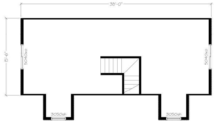
Possible 2nd Floor Plan
